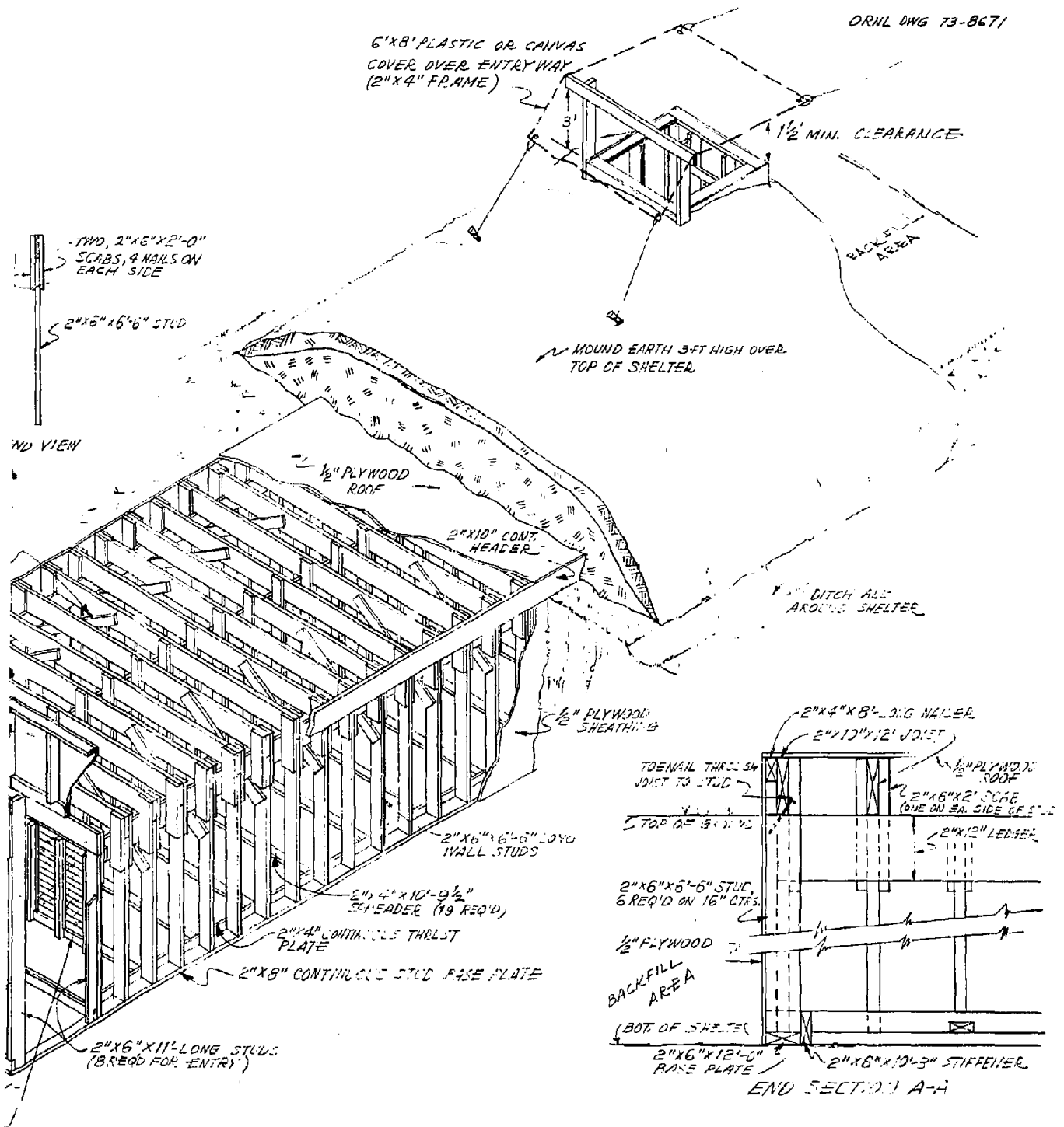
fig. A-7.1. Rigid Frame Underground, Pictorial View.
